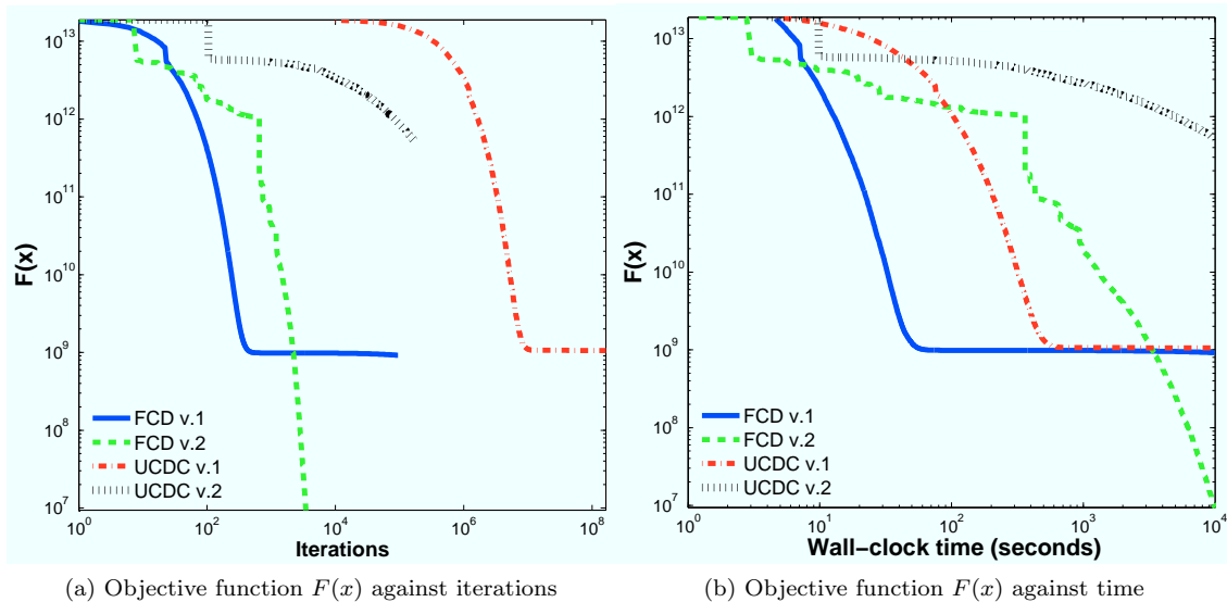
Figure 1: Performance of all four methods FCD v.1 and v.2 and UCDC v.1 and v.2 on a sparse large scale \ell_1 -regularized least squares problem. For practical purposes, for UCDC v.1 results are printed every ten thousand iterations. Calculation of F(x) is not included in running time of the methods. Fig.1a shows how the objective function F(x) decreases as a function of the number of iterations. Fig.1b shows how the objective function F(x) decreases as a function of wall-clock time measured in seconds.
