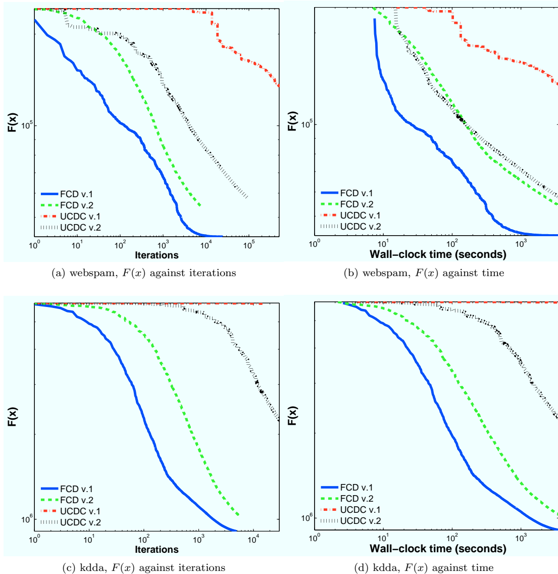
Figure 2: Performance of all four methods FCD v.1 and v.2 and UCDC v.1 and v.2 on two large scale \ell_1 -regularized logistic regression problems. The first and second rows of figures show the results for problems webspam and kdda , respectively. Calculation of F(x) is not included in running time of the methods.
